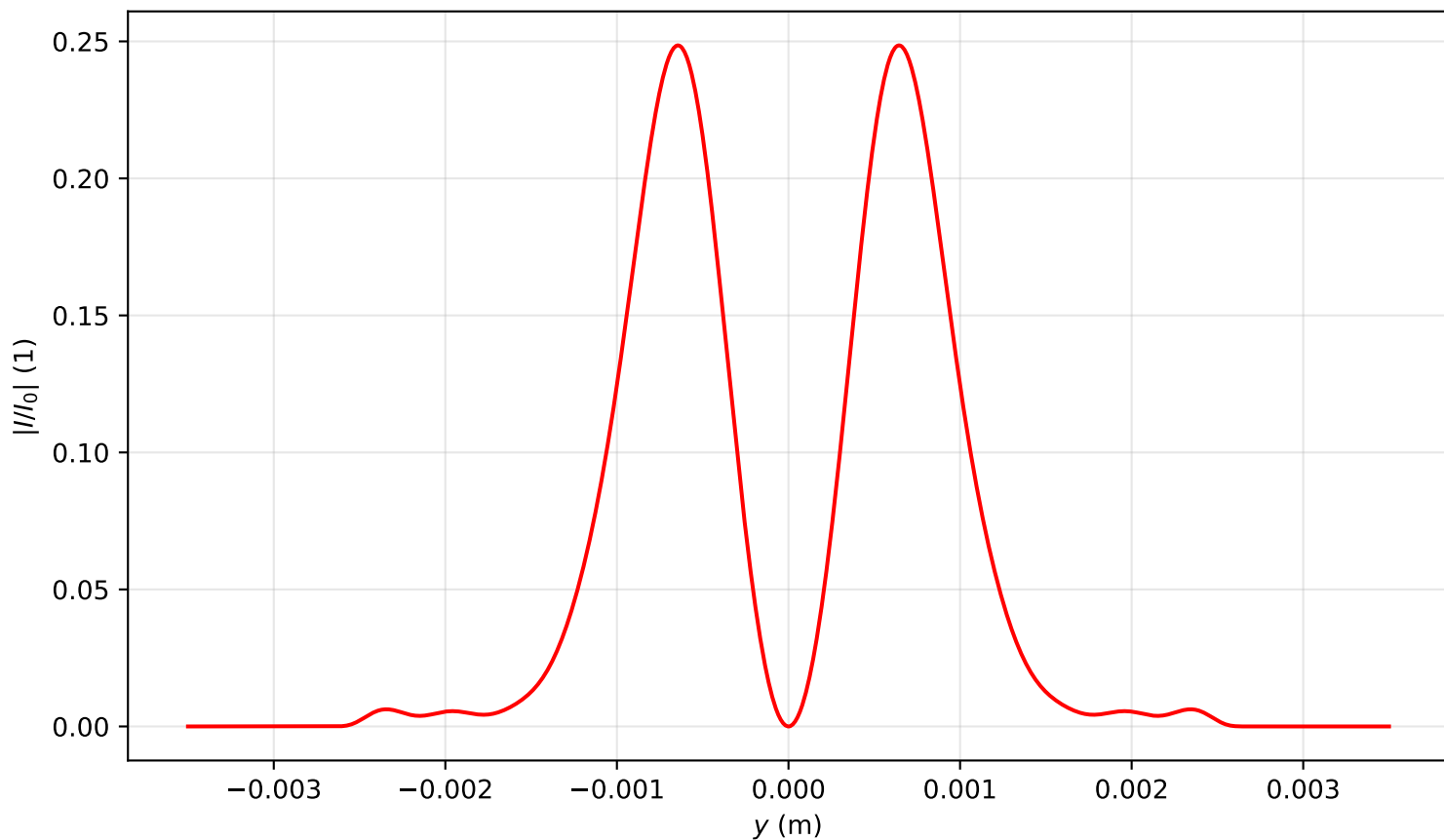
Intensity profile I(x=0, y, z=2.468)/I_0 , \text{Pin}=4.0\text{Pcr} , artificial time
